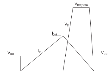
Figure 19: Unclamped inductive waveform
