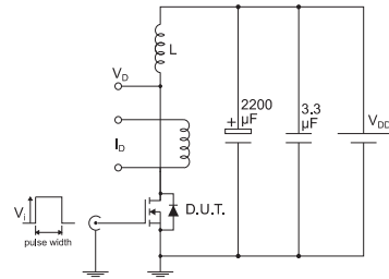
Figure 18: Unclamped inductive load test circuit
