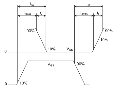
Figure 20: Switching time waveform
