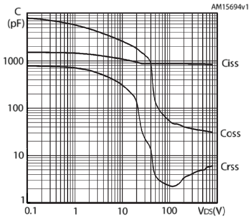
Figure 8: Capacitance variations
